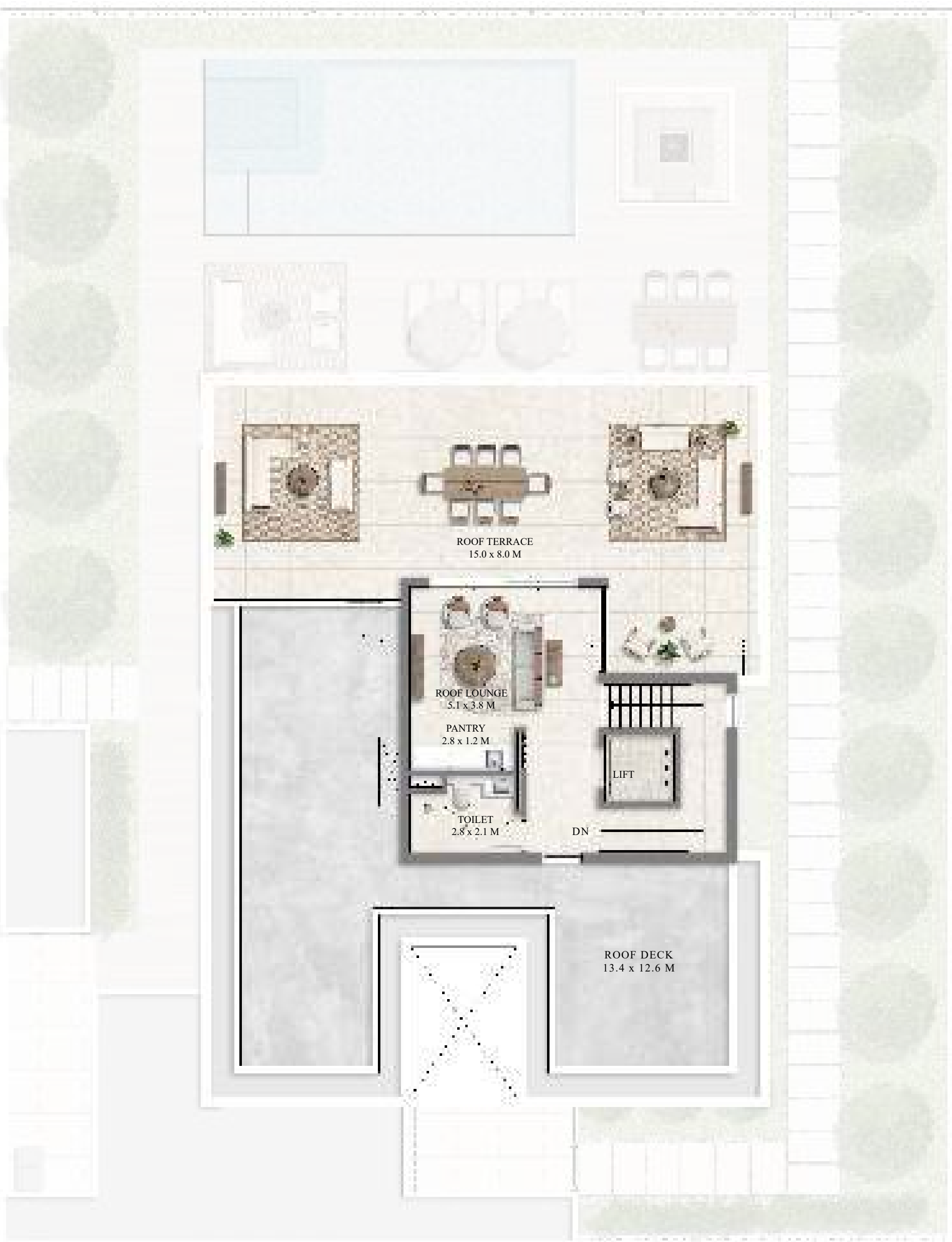
SECOND FLOOR
