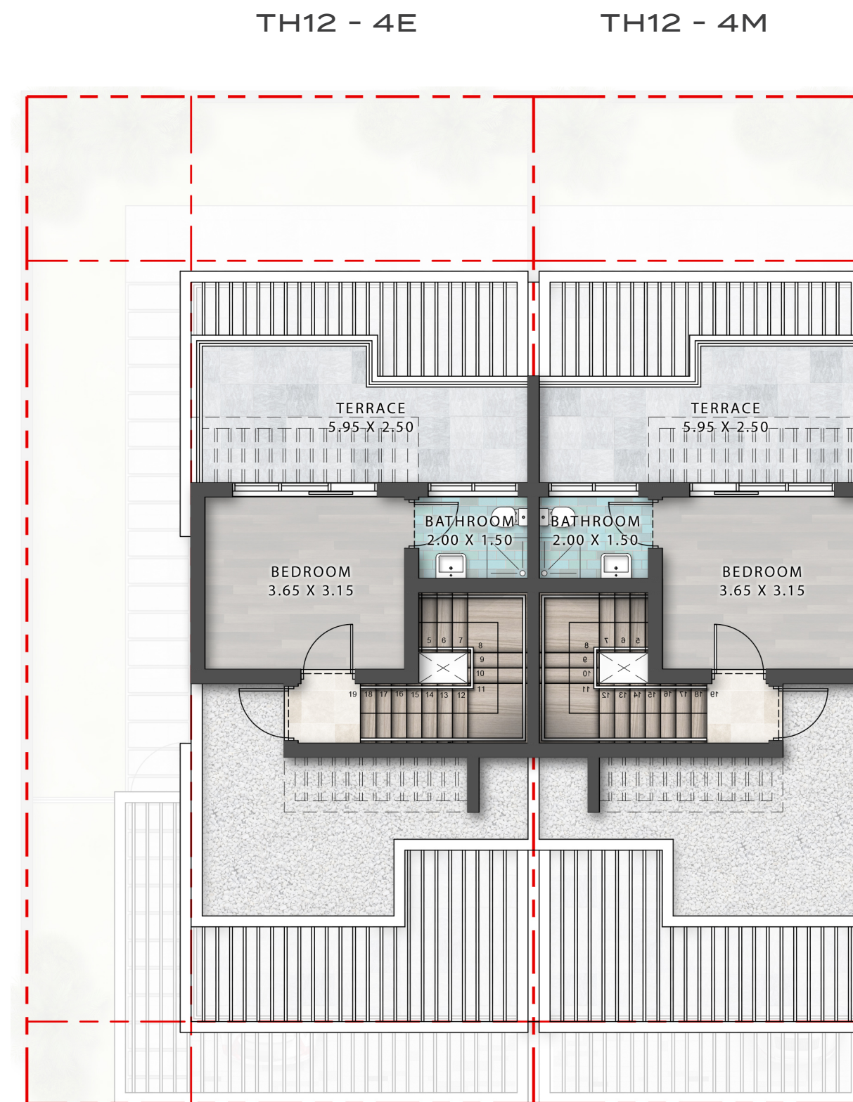
ROOF FLOOR
