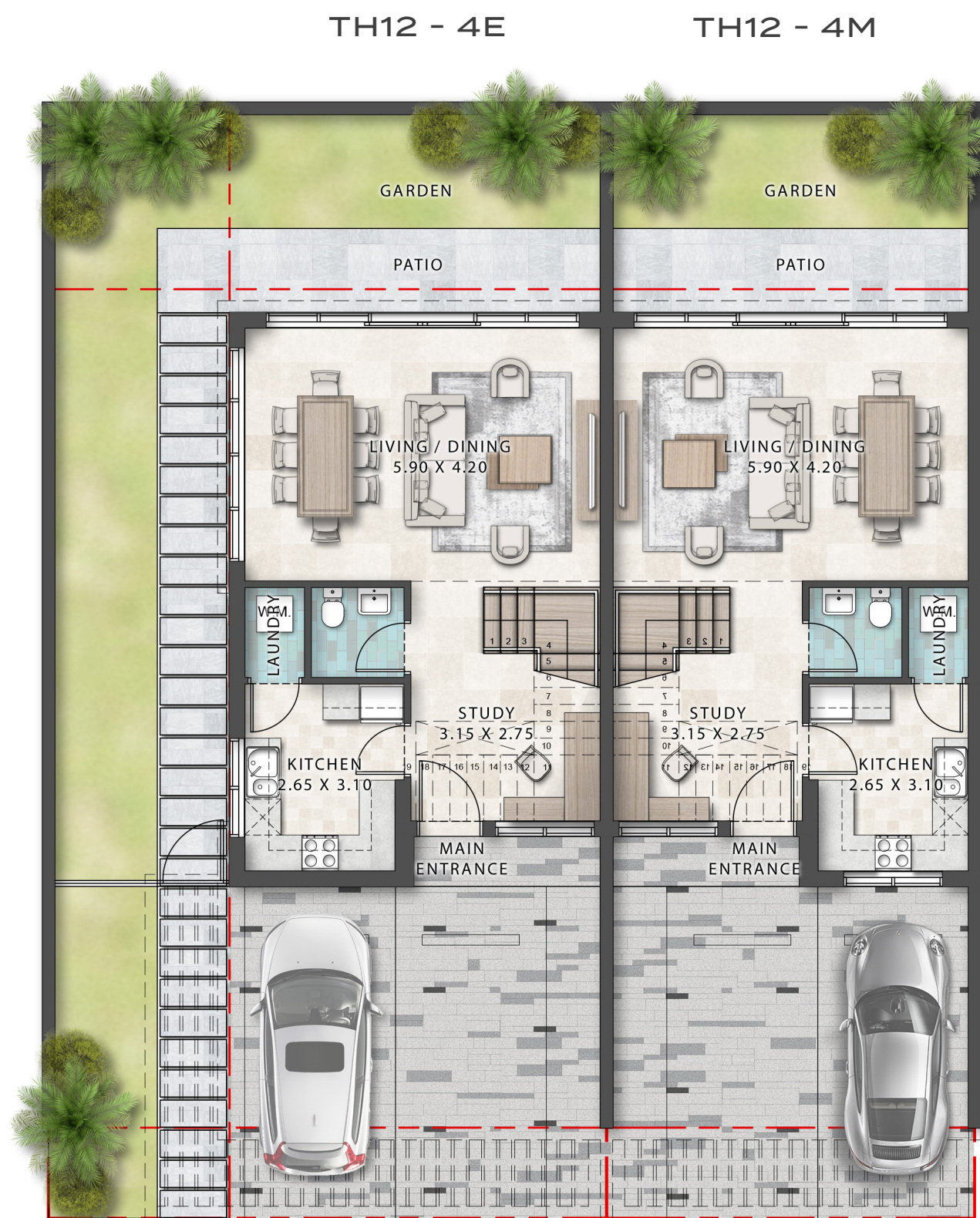
GROUND FLOOR
