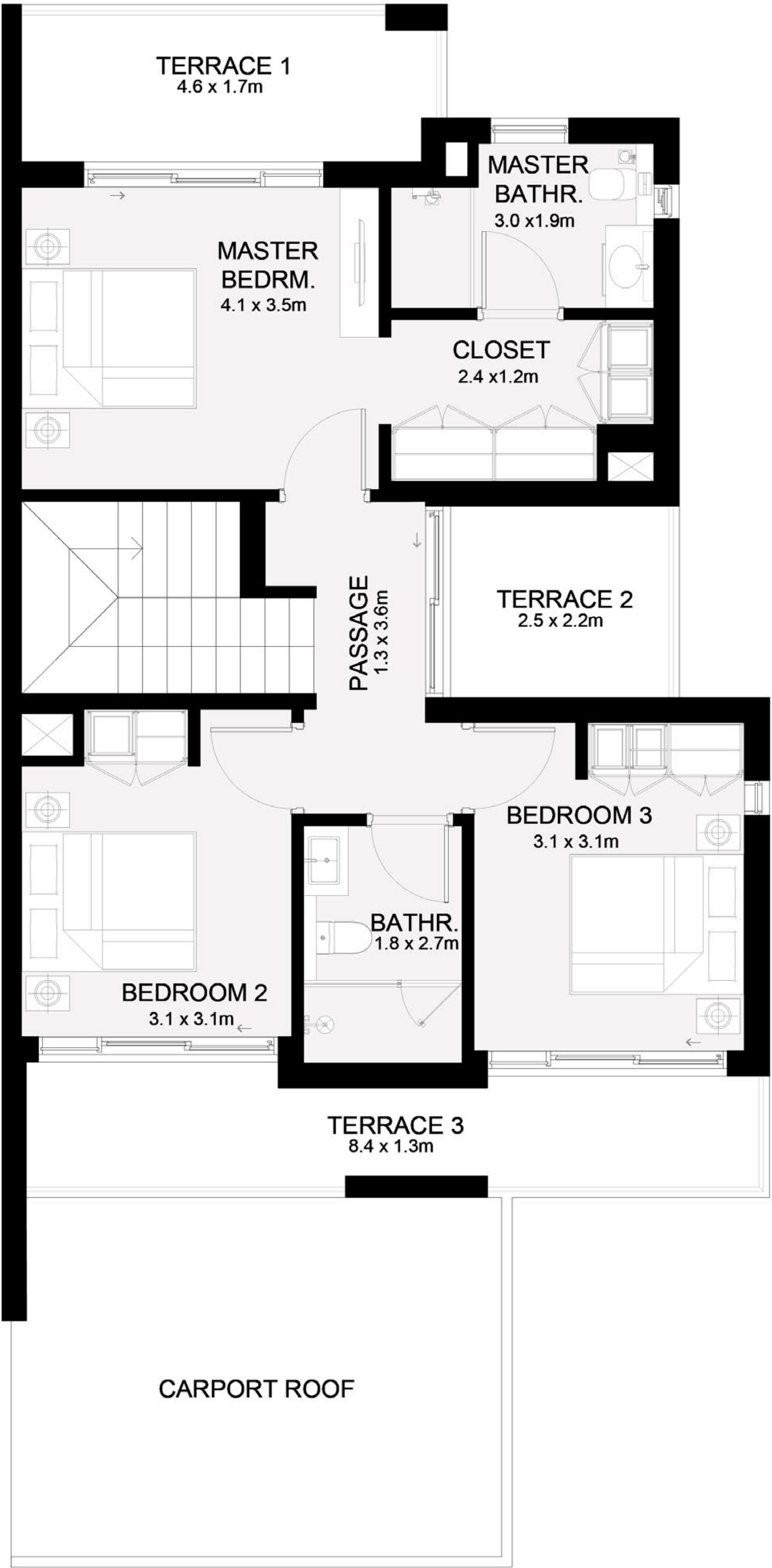
FIRST FLOOR
