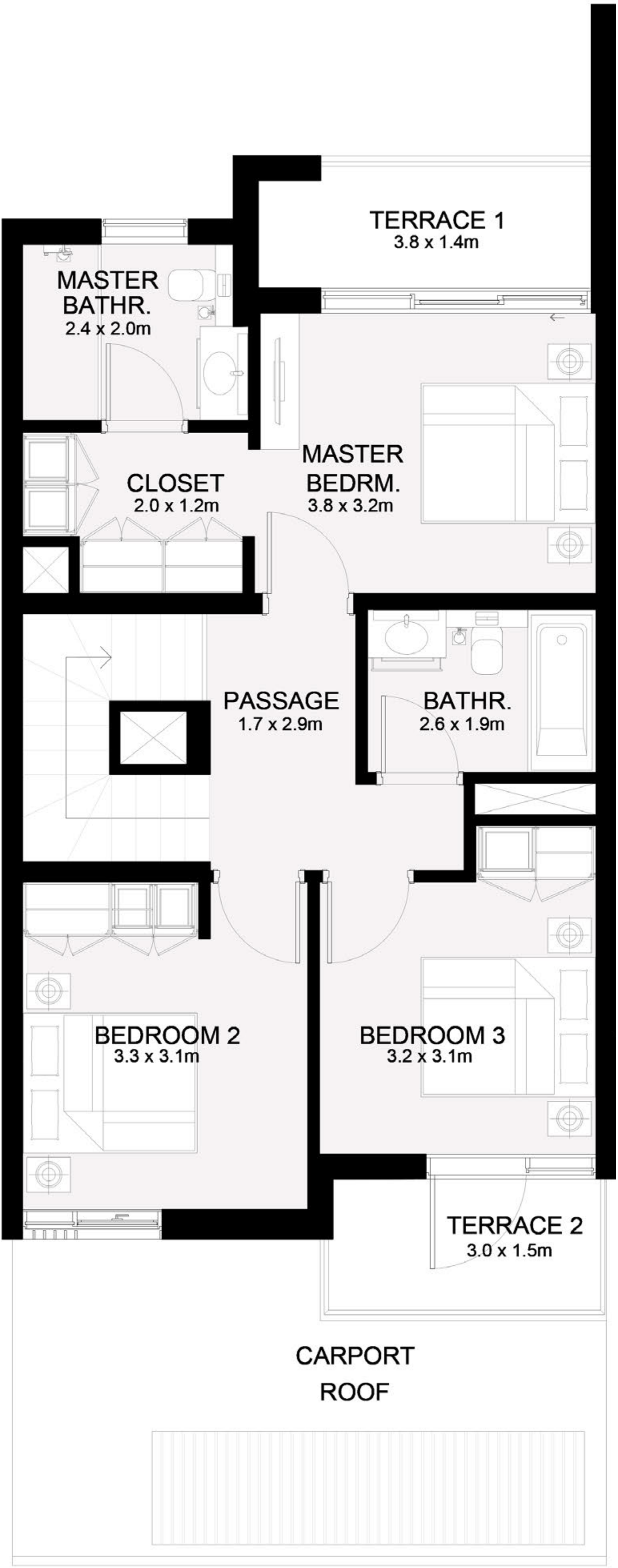
FIRST FLOOR
