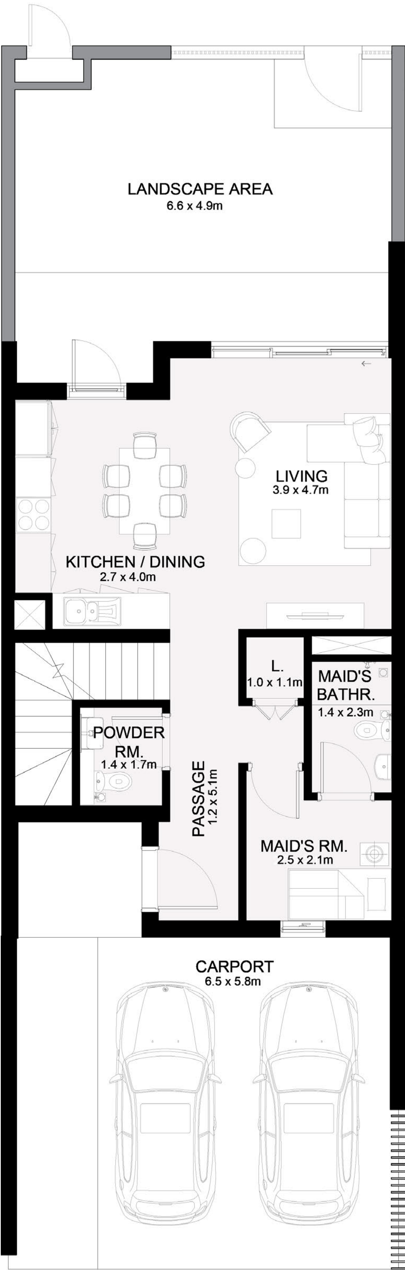
GROUND FLOOR
