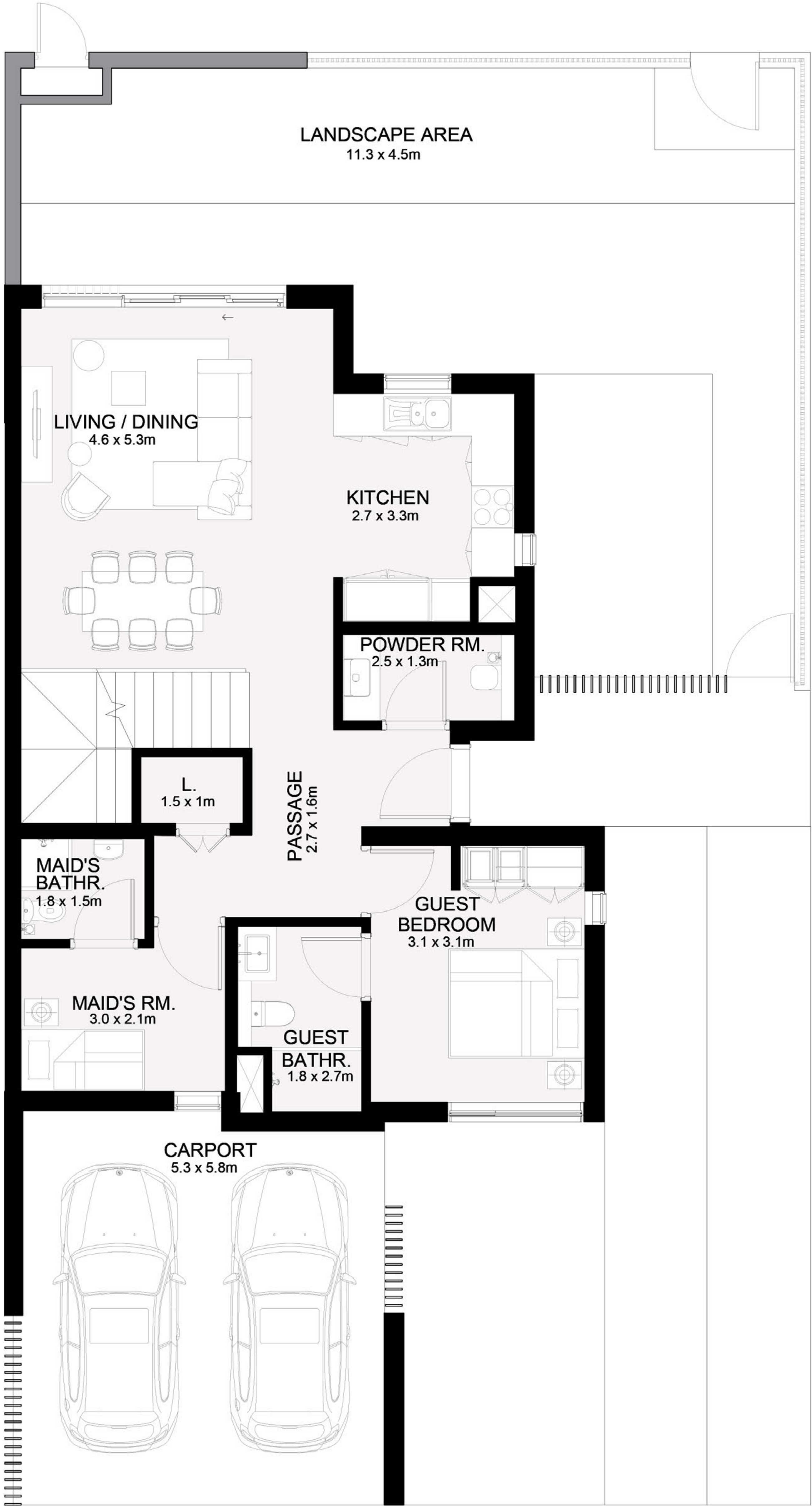
GROUND FLOOR
