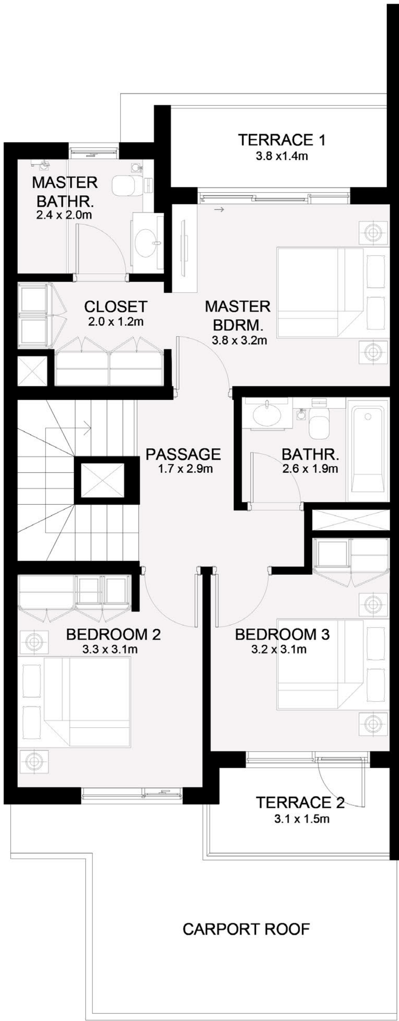
FIRST FLOOR
