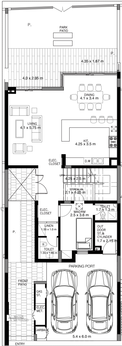
Ground Floor
