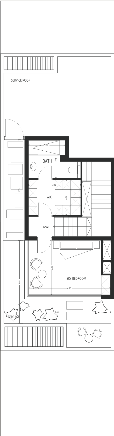
SECOND FLOOR
