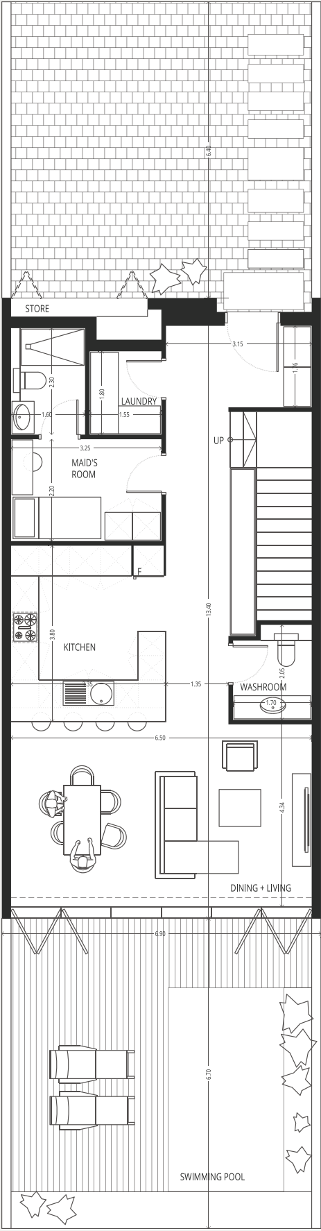
GROUND FLOOR
